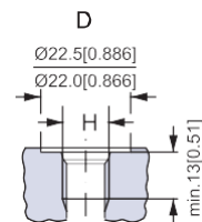
D: UNF drain port H: 9/16 - 18 UNF
