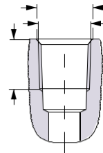
C: NPTF main ports I: ½ - 14 NPTF
