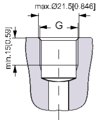
A: G main ports G: ISO 228/1 - G 1/2
