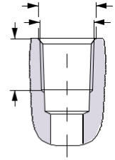
C: NPTF main I: 1/2 - 14 NPTF
